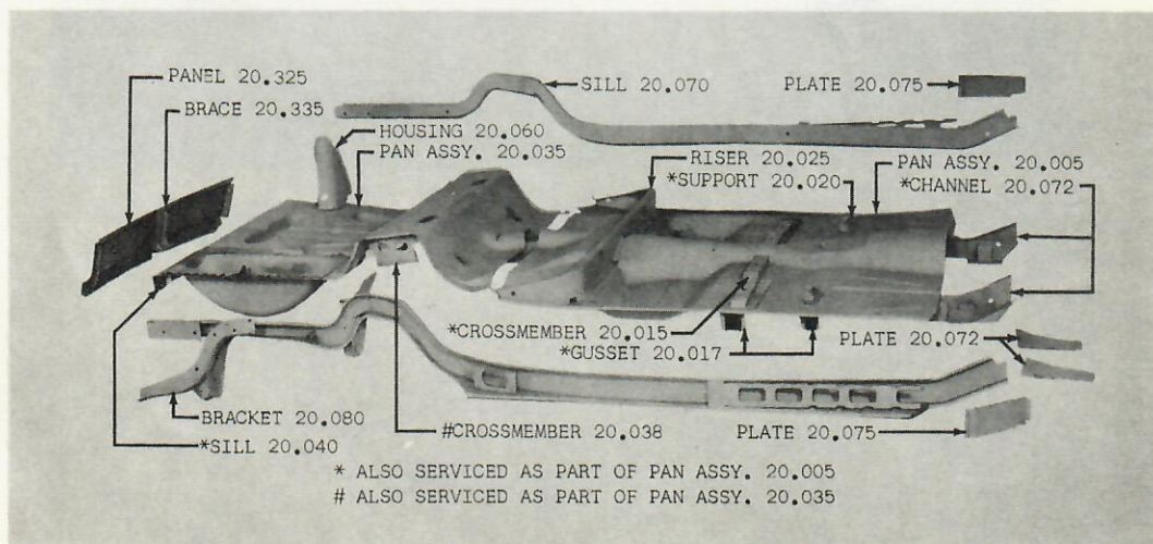
GROUP 20 - FIG. 2 - UNDERBODY PANELS 10-20-80
