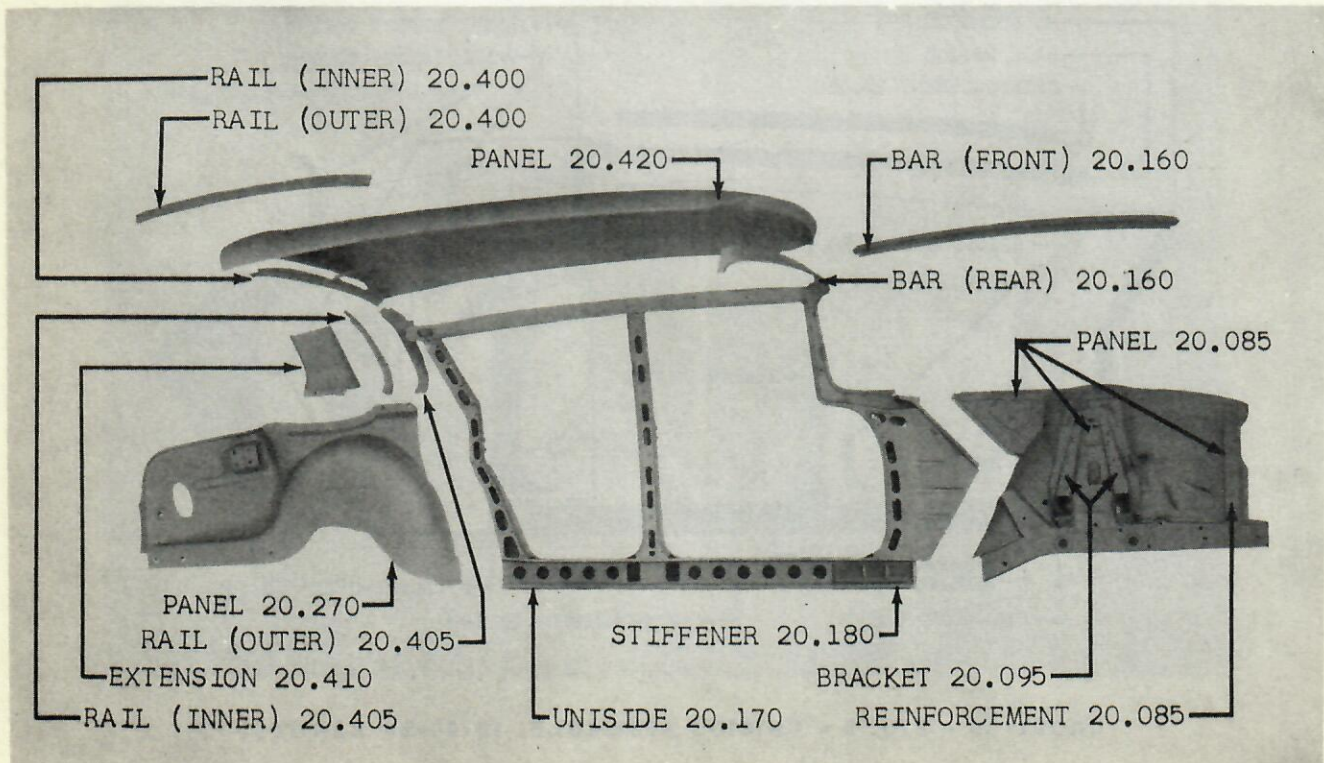
GROUP 20 - FIG. 7 - BODY SIDE PANELS 10-20-80 SEDAN
