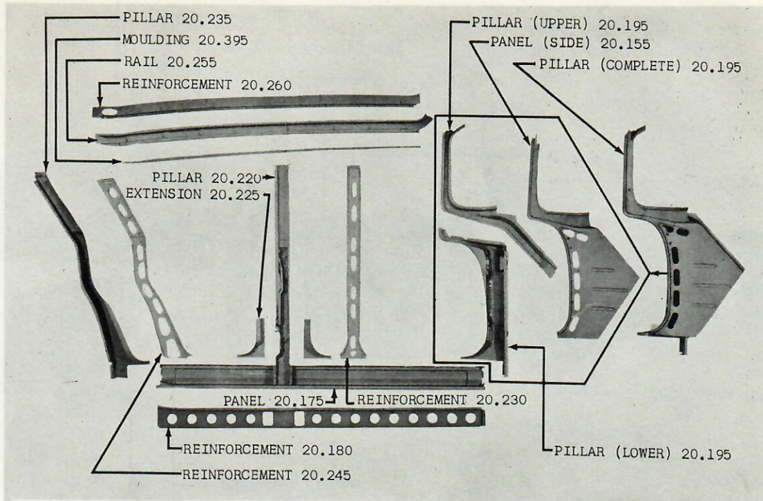
GROUP 20 - FIG. 4 - UNISIDE ASSEMBLY 10-20-80 SEDAN
