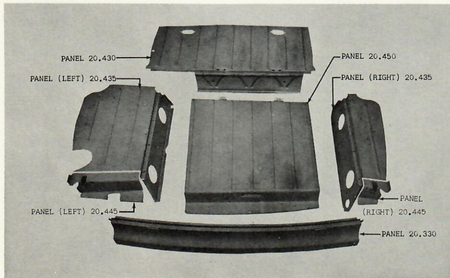
GROUP 20 - FIG. 10 - AUXILIARY FLOOR PANELS 10-20-80 STATION WAGON
