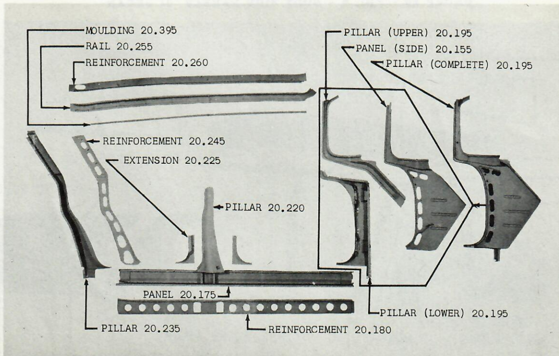
GROUP 20 - FIG. 5 - UNISIDE ASSEMBLY 10-20-80 HARDTOP
