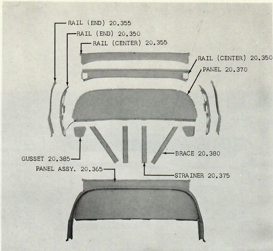
GROUP 20 - FIG. 9 - REAR SHELF PANELS 10-20-80 SEDAN
