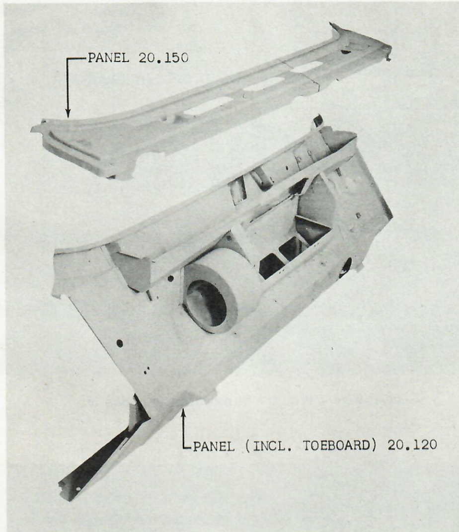
GROUP 20 - FIG. 3 - DASH PANEL 10-20-80
