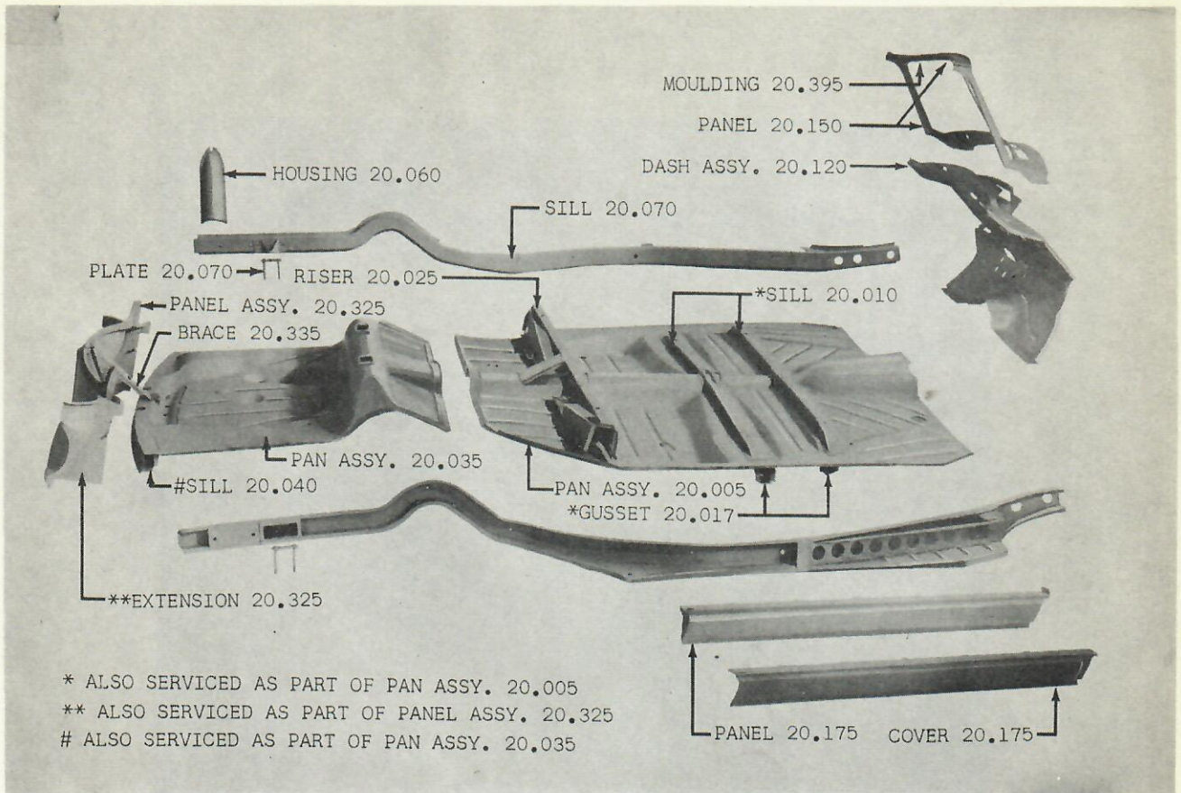
GROUP 20 - FIG. 1 - UNDERBODY PANELS 01
