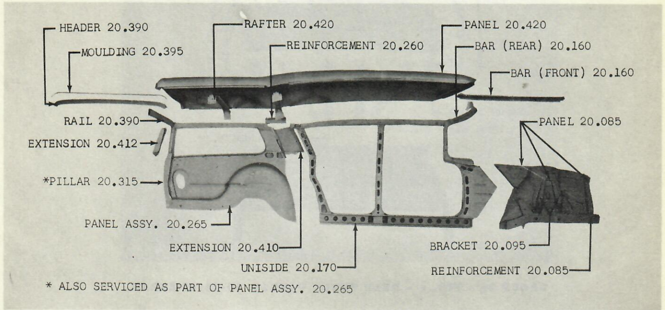
GROUP 20 - FIG. 8 - BODY SIDE PANELS 10-20-80 STATION WAGON
